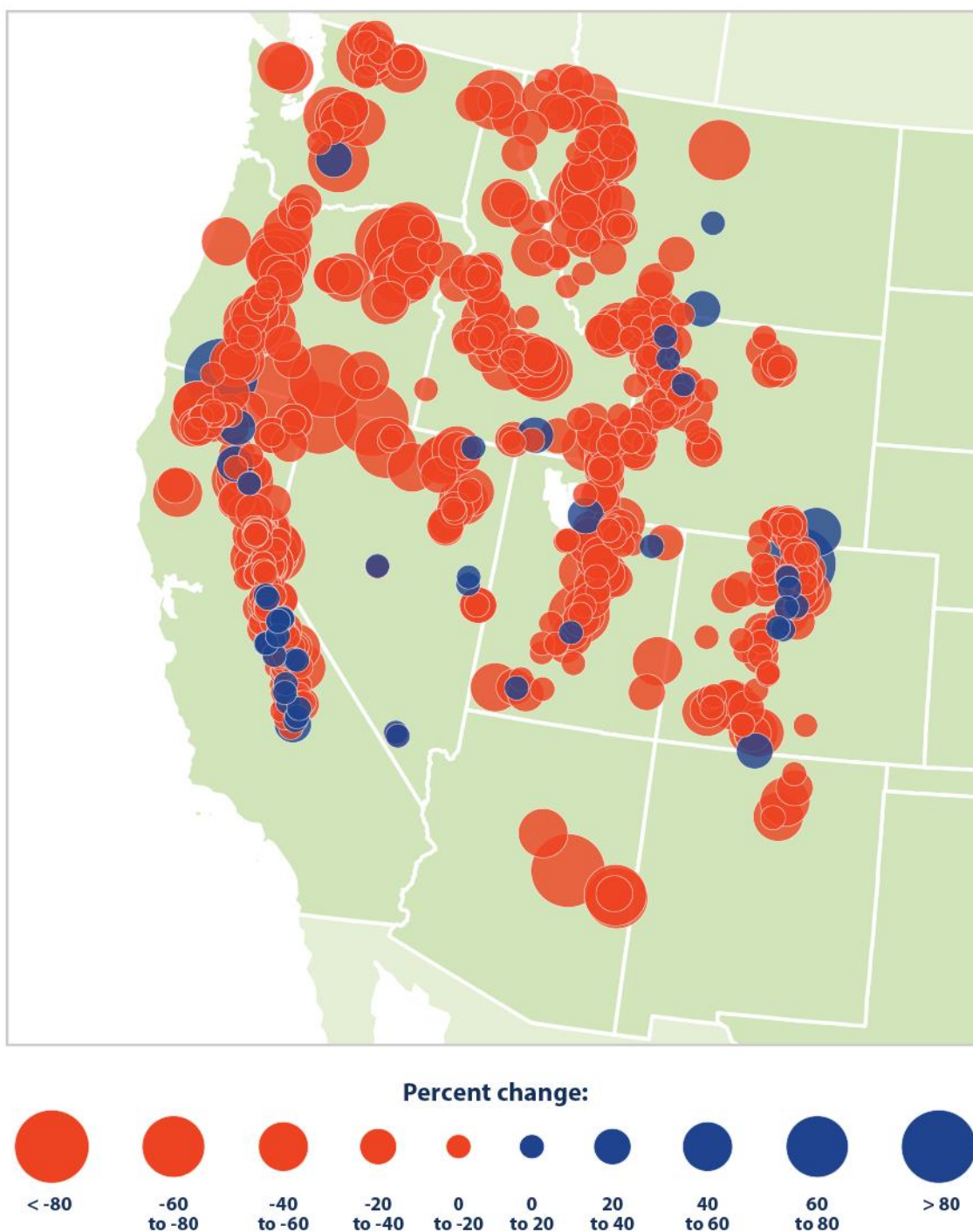
Figure 1: Trends in April snowpack in mountains of the western United States, 1955-2016. Data source: Mote, P.W. and D. Sharp 2016 update to data originally published in Mote et al. 2005. Retrieved from the U.S. EPA's "Climate Change Indicators in the United States," www.epa.gov/climate-indicators .
