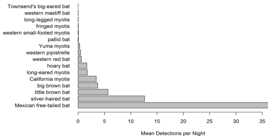
Figure 5. Mean detections per night for bat species detected in the Storrie and Chips fire study area in 2015-16.
