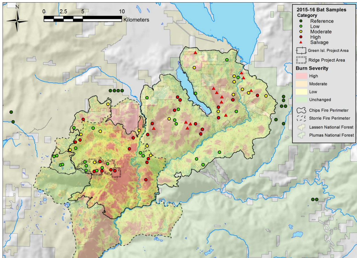
Figure 2. Locations where automated recorder units were deployed in the Storrie and Chips Fire areas to sample the calls of bats.
