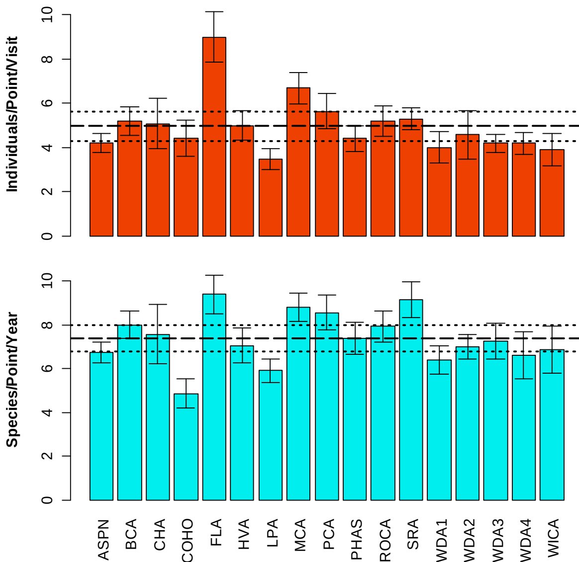
Figure 1-2. Total avian abundance (top panel) and avian species richness (bottom panel) at 17 aspen sites in the northern Sierra Nevada in 2011 ( \pm SE). Dashed lines represent the mean for all sites combined and dotted lines the 95% confidence interval surrounding that estimate. Four-letter transect codes are defined in Table 1-1.
